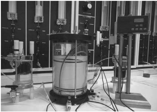
Figure 2. Flexible-wall hydraulic conductivity cell provided with bender elements and a cathetometer
