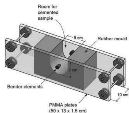
Figure 1. Bench top bender element setup
