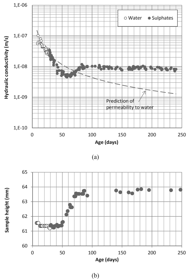
Figure 4. Impact of sulphate attack on the (a) hydraulic conductivity and (b) the height of a cement-bentonite sample during permeation with water and a 25 g/L \text{Na}_2\text{SO}_4 solution in a flexible wall cell.
