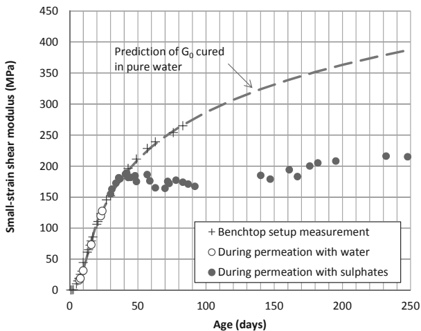
Figure 3. Impact of sulphate attack on the small-strain shear modulus of a cement-bentonite sample
