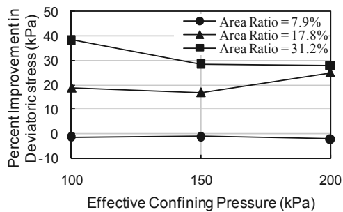
Figure 6. Dependency of the percent improvement in deviatoric stress at failure on the effective confining pressure
