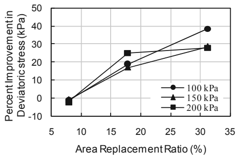
Figure 7. Dependency of the percent improvement in deviatoric stress at failure on the area replacement ratio.
