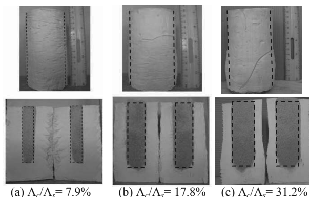
Figure 2. Internal and external modes of failure.
