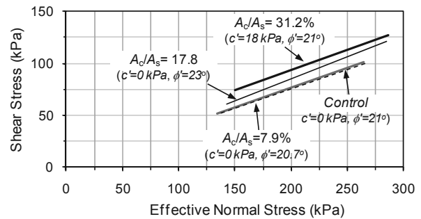
Figure 8. Failure envelopes for control and reinforced clay specimens.
