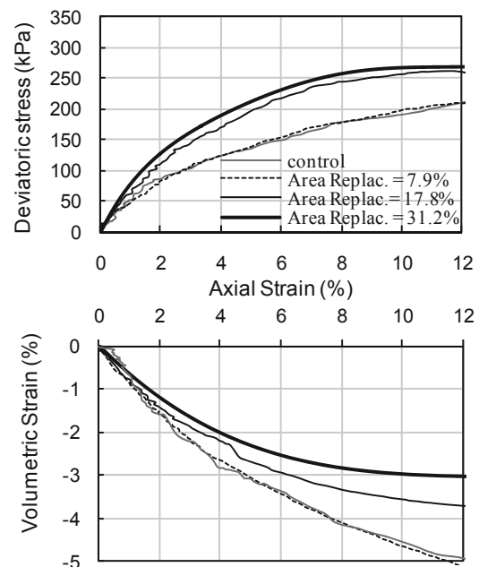
Figure 5. Variation of deviatoric stress and volumetric strain with axial strain ( A_c/A_s=31.2\% ).
