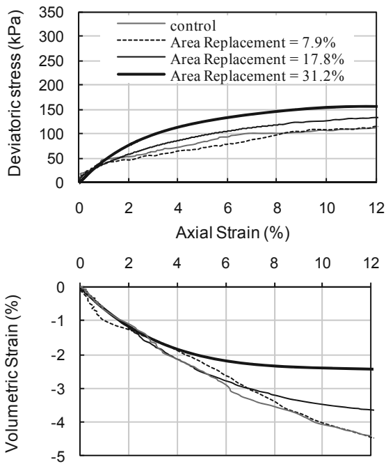
Figure 3. Variation of deviatoric stress and volumetric strain with axial strain ( A_c/A_s=7.9\% ).
