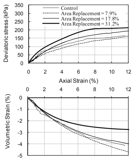
Figure 4. Variation of deviatoric stress and volumetric strain with axial strain ( A_c/A_s=17.8\% ).
