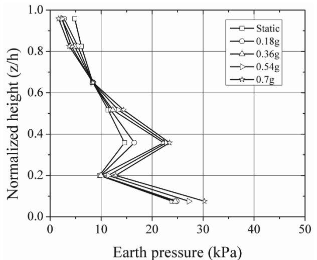
Figure 6. Earth pressure distribution for experiments without geofoam inclusion
