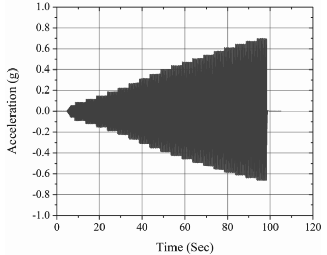
Figure 5. Stepped-amplitude sinusoidal excitation input
