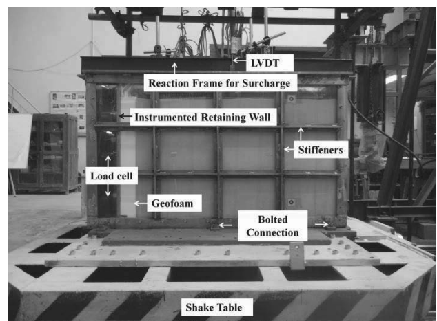
Figure 2. Pictorial view of experimental setup
