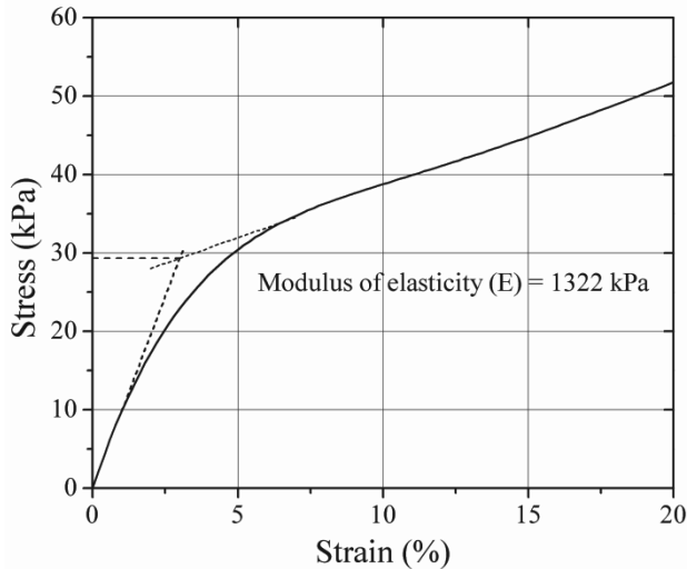
Figure 3. Stress-strain behavior of 10D EPS geofoam
