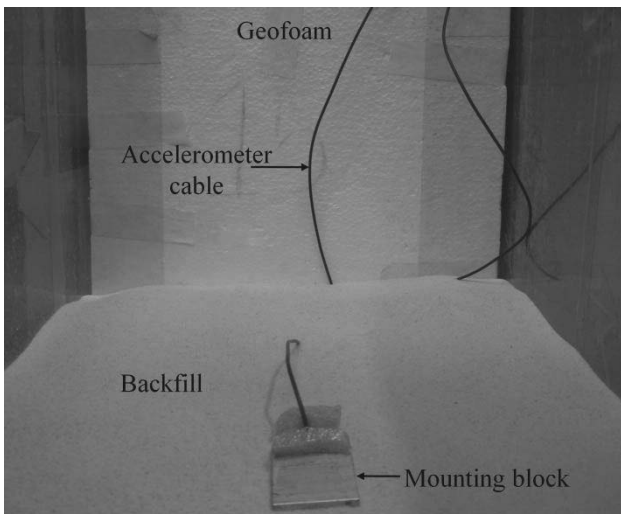
Figure 4. Positioning of Accelerometer in the backfill
