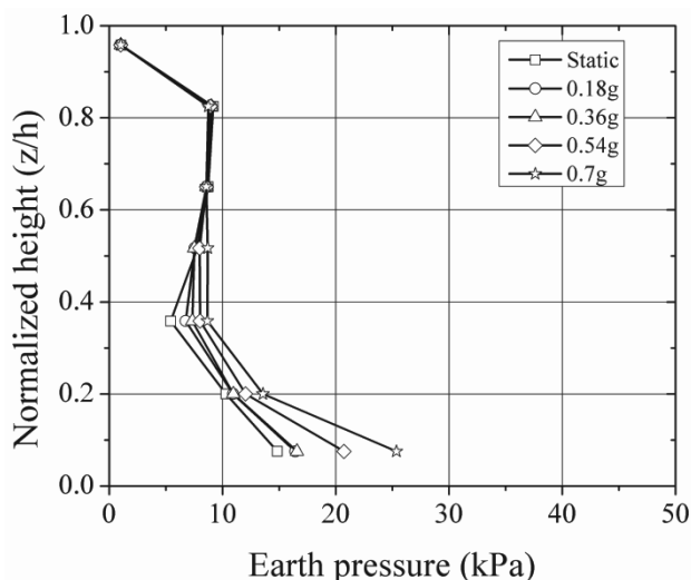
Figure 7. Earth pressure distribution for experiments with geofoam inclusion
