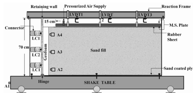
Figure 1. Detailed diagram of experimental setup
