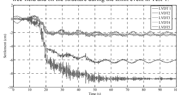
Figure 10. Settlement recorded at various locations with respect to the structure in Test-1 during the Izmit event.
