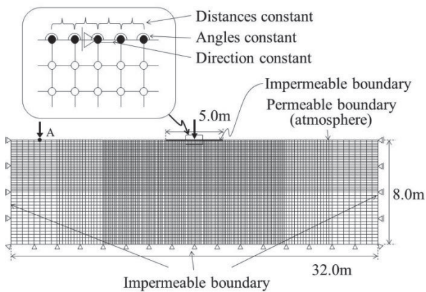
Figure 1. Finite element mesh and boundary conditions.
