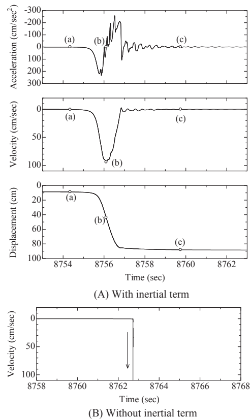
Figure 6. Time history of acceleration, velocity, and displacement of the central node of the foundation (load controlled case)
