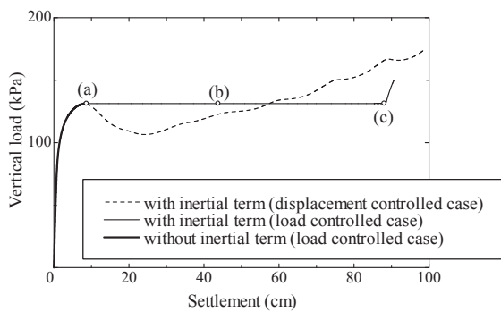
Figure 4. Relationship between vertical load and settlement (load controlled case)
