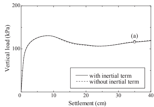
Figure 2. Relationship between vertical load and settlement (displacement controlled case).
