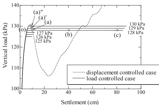
Figure 7. Relationship between vertical load and settlement (load constant case)
