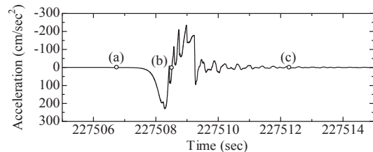
Figure 10. Time history of acceleration of central node of foundation (load: 128 kPa)
