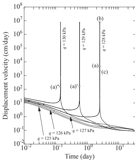
Figure 8. Relationship between time and displacement velocity (load constant case)
