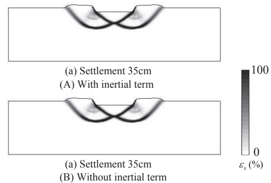
Figure 3. Shear strain distributions (displacement controlled case).
