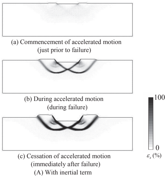
Figure 5. Shear strain distributions (load controlled case)
