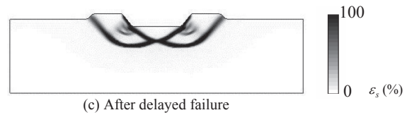
Figure 9. Distribution of shear strain (load: 128 kPa)
