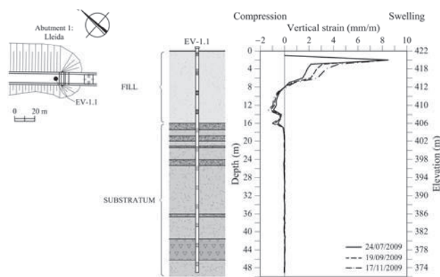
Figure 2. Vertical strains measured by sliding micrometer EV-1.1
