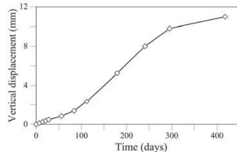
Figure 7. Accumulated vertical displacements measured by a continuous extensometer
