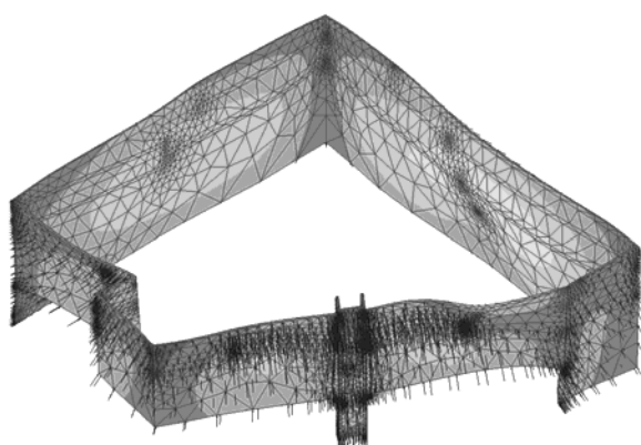
Figure 4. Deformed shape of the sheet pile wall with deflection vectors. (Deformed shape is scaled to 200 times).
