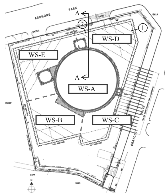
Figure 1. Plan view of the project site with strutting system
