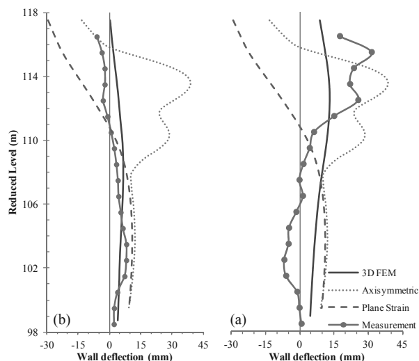
Figure 3. Deflection profiles of sheet pile wall: (a) at section 1, and (b) at section 2. Section 1 and 2 are as shown in Figure 1.
