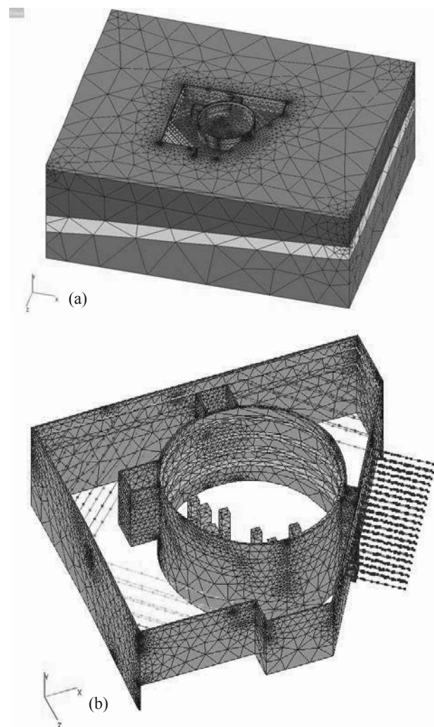
Figure 2. Finite element mesh: (a) Overall geometry, and (b) Structural elements and strutting system
