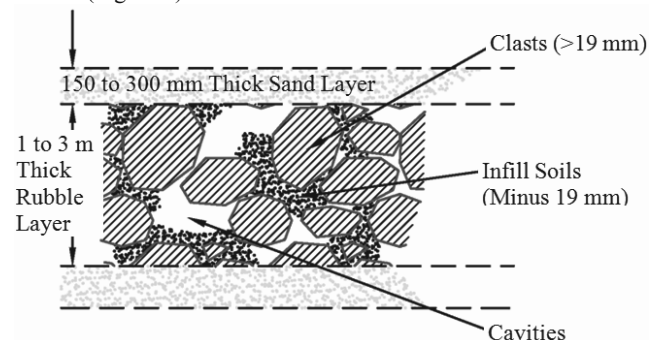
Figure 2. Debris Fill Structure
