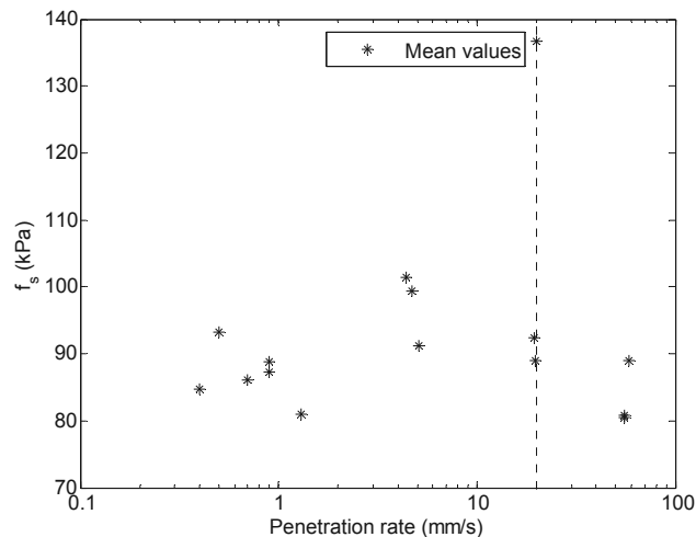
Figure 5. The mean sleeve friction plotted against the mean penetration rate from 4.5 to 11.4 m below ground level. No correlation seems to exist. The standard rate of penetration of 20 mm/s has been marked with a dotted line.
