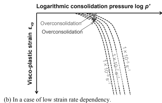
Figure 7. Illustration of long-term consolidation settlement in overconsolidation domain.
