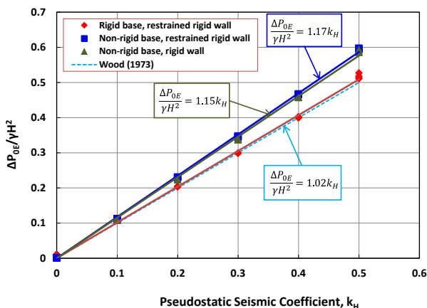
Figure 4. The relationship of normalized total increment of seismic earth pressure versus seismic coefficient for various conditions.
