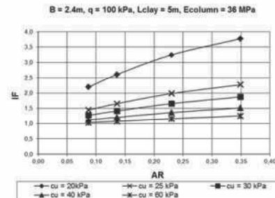
Figure 12. Settlement improvement factor (IF) vs. area ratio (AR) charts for a rigid square footing ( B=2.4m ) with a foundation pressure of q=100 kPa resting on end bearing rammed aggregate piers ( L=5m, E=36 MPa)
