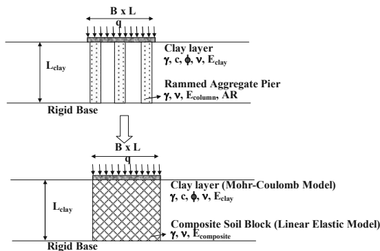
Figure 11 Schematic representation of composite soil model
