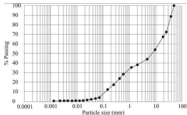
Figure 2. RCDW grain size distribution (Santos et al. 2010).
