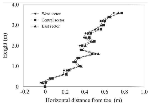
Figure 7. Post-construction face profile (Santos et al. 2010).
