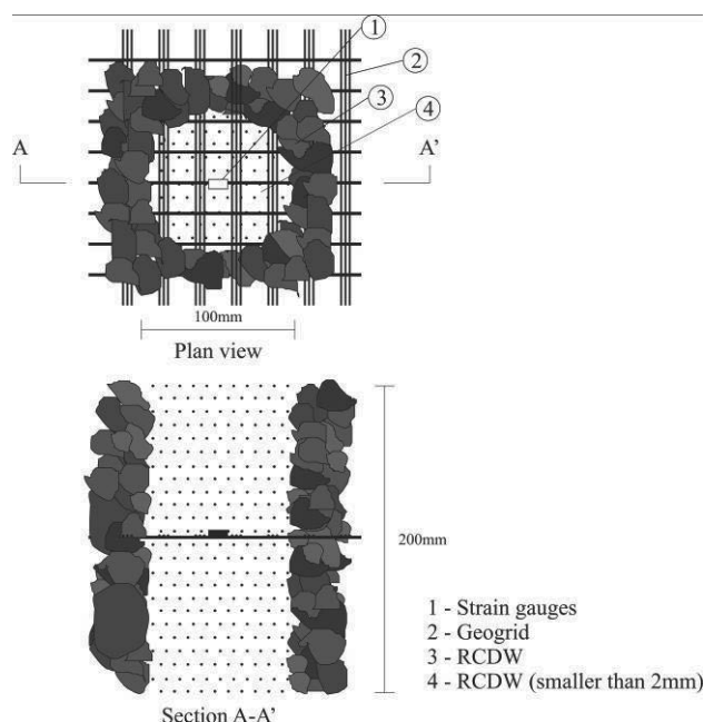
Figure 6. Region around strain gauges (wall #1).
