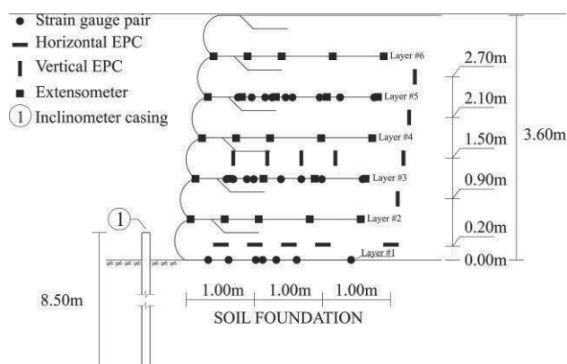
Figure 5. Instruments distribution profile.
