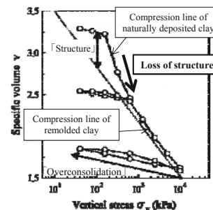
Figure 1. One-dimensional compression of natural deposited clay and definition of structure and overconsolidation
