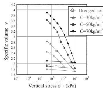
Figure 5. Standard consolidation test results for 3 remolded treated soils
