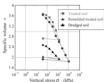
Figure 2. Comparison of uniaxial compression properties of treated soil, remolded treated soil, and dredged soil
