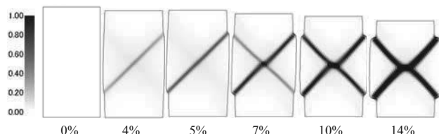
Figure 11. Consolidated undrained triaxial analysis results for remolded treated soil
