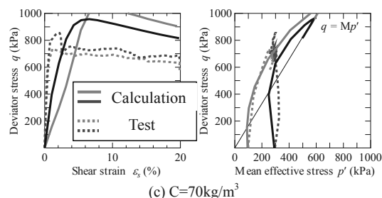
Fig. 8 Consolidated undrained triaxial test results for treated soil and their analytical reproduction
