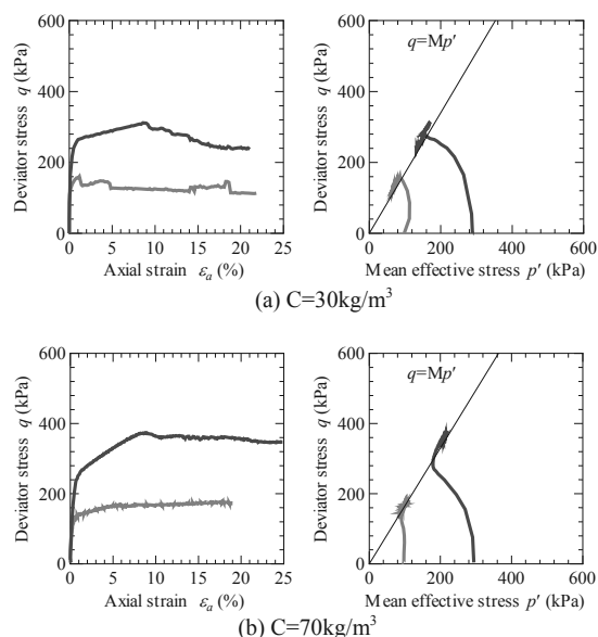
Figure 6. Consolidated undrained triaxial compression test results for remolded treated soils
