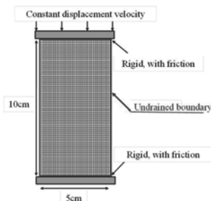
Figure 9. Finite element mesh and boundary conditions
