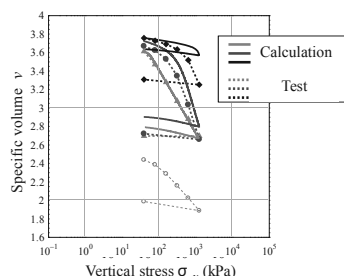
Figure 7. Treated soil standard consolidation test results and their analytical reproduction
