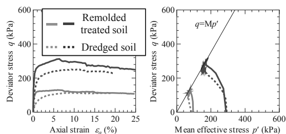
Figure 4. Consolidated undrained triaxial test results for remolded treated soil
