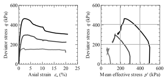
Figure 3. Consolidated undrained triaxial test results for treated soil
