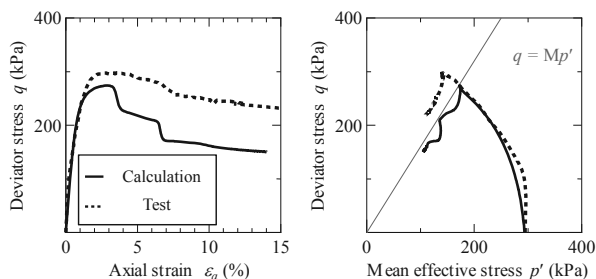
Figure 10. Consolidated undrained triaxial test results for remolded treated soil
