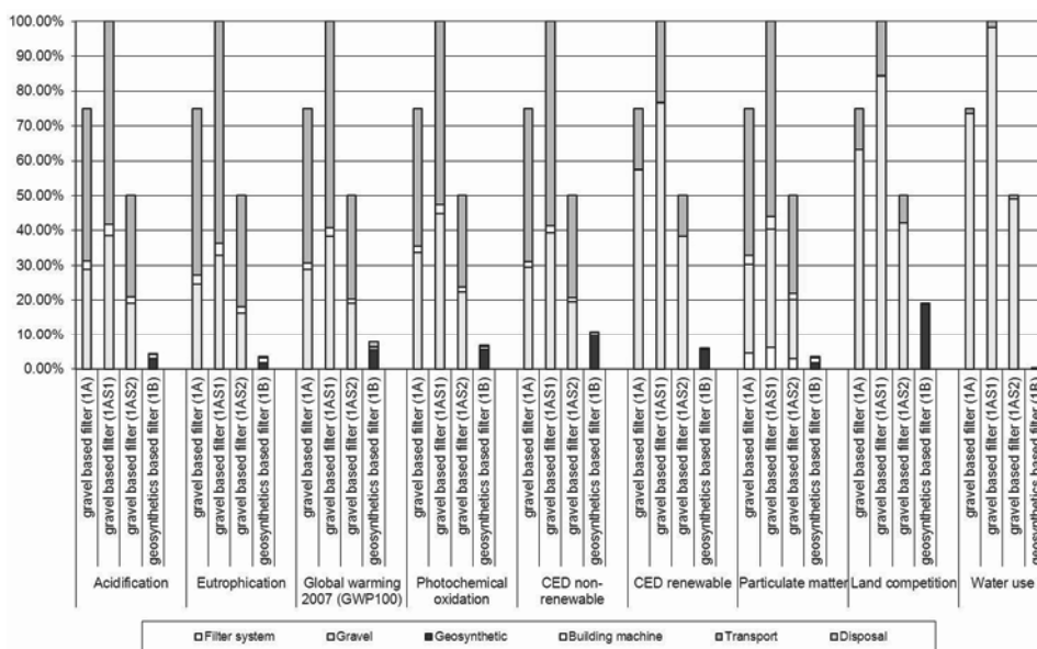
Figure 2. Sensitivity analysis: environmental impacts of the life cycle of 1 m 2 of filter layer. 1AS1 and 1AS2 refer to the sensitivity analysis with a different thickness of the gravel based filter layer. For each indicator, the case with highest environmental impacts is scaled to 100%.
