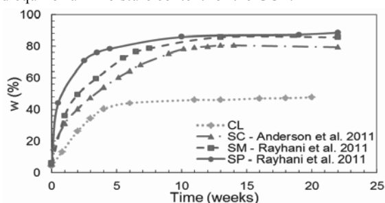
Figure 3. Hydration response of GCL2 from different subsoils at w_{fdn}=10\% initial moisture content (CL: Clay, SC: clayey sand, SM: silty sand, SP: poorly graded sand)
