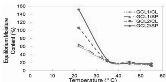
Figure 6. GCL moisture uptake vs. temperature (Barclay & Rayhani, 2012)
