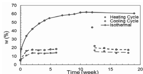
Figure 4. Effect of daily and seasonal thermal cycles on hydration of GCL2 (subsoil=CL, w_{fdn}=30\% ) (Sarabiam and Rayhani, 2012)
