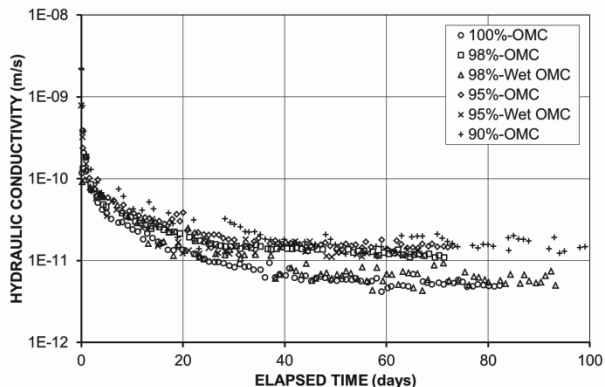
Figure 3. Hydraulic conductivity of SB3 specimens compacted to various dry densities at various moisture contents.
