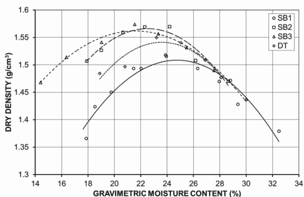
Figure 1. Compaction curves for clay samples.
