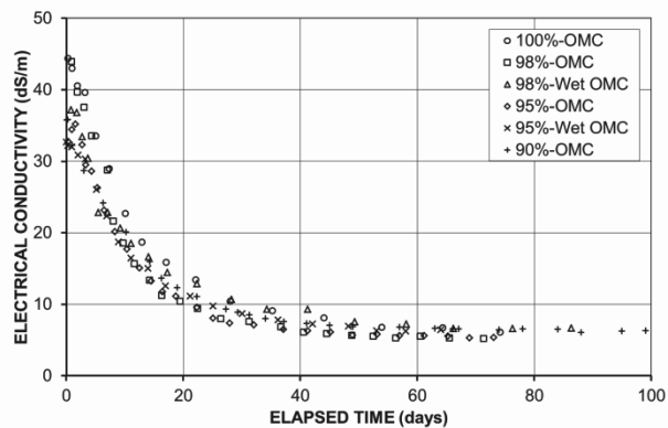
Figure 4. Electrical conductivity of SB3 specimens compacted to various dry densities at various moisture contents.
