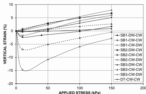
Figure 8. Vertical strains measured during oedometer tests.
