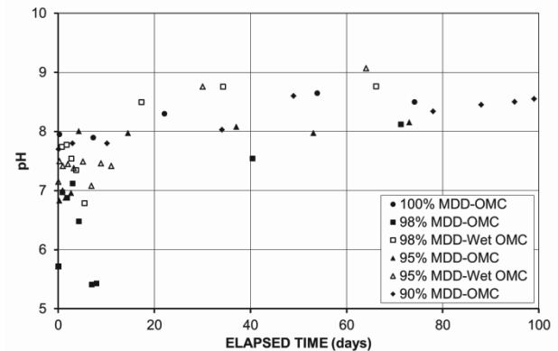
Figure 6. pH of SB3 specimens compacted to various dry densities at various moisture contents.
