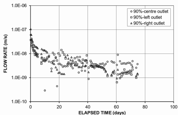
Figure 2. Flow rates from centre and outer outlets during testing of 90% MDD at OMC specimen with roughened permeameter wall.
