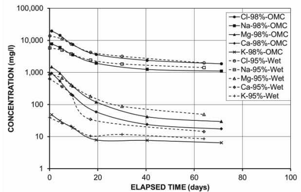
Figure 5. Concentrations of major ions in outflow from SB3 specimens compacted to 98% and 95% of MDD.
