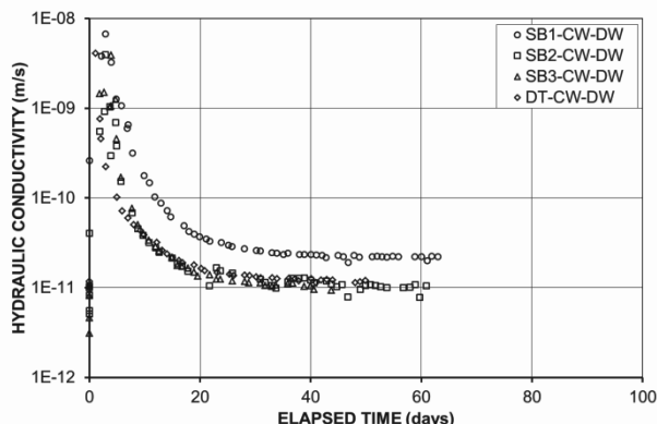
Figure 7. Hydraulic conductivity of all specimens moisture-conditioned with CW, compacted, and permeated with DW.
