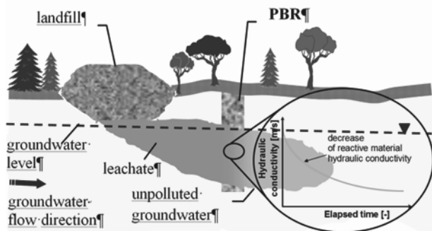
Figure 1. A concept of permeable reactive barriers.
