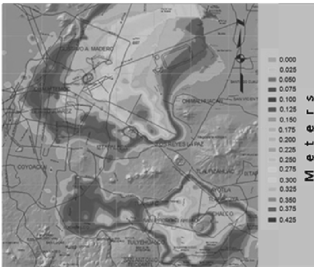
Figure 5. Subsidence rate in m/year during the 1998-2002 period.
