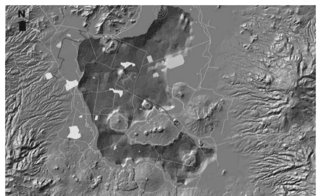
Figure 4. Relief of the former lakes of Mexico Valley.
