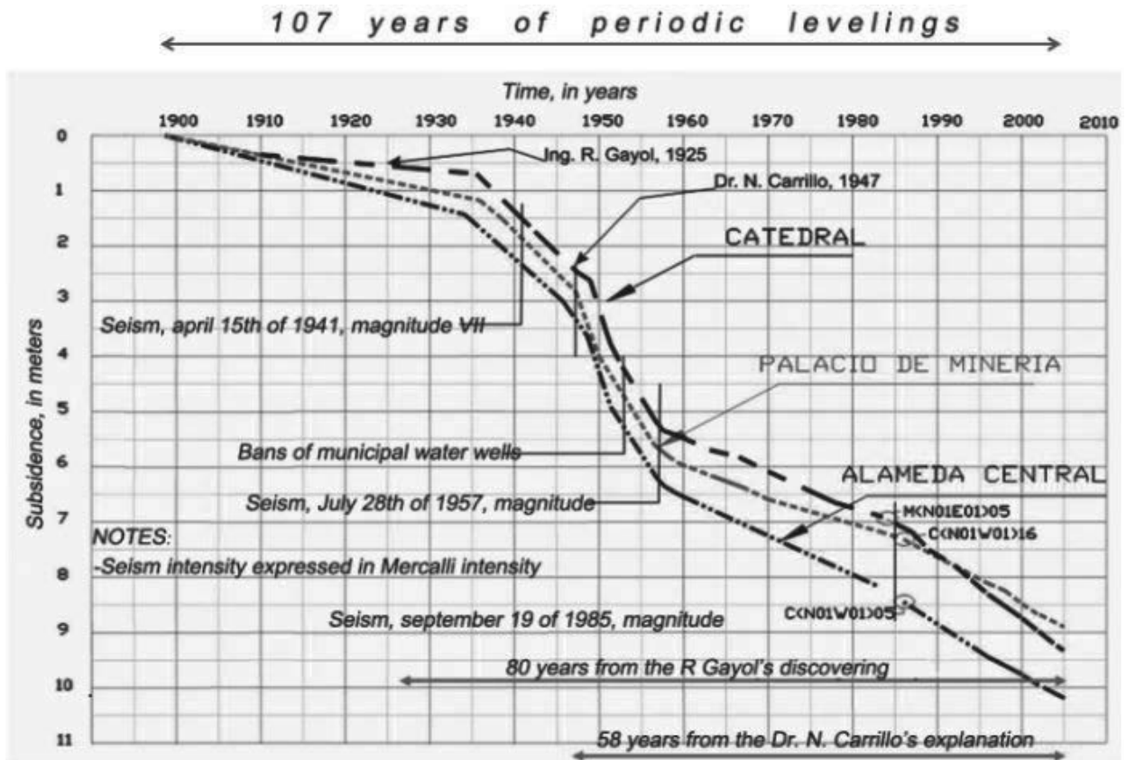
Figure 2. Local evolution of subsidence for the 1898-2005 period.
