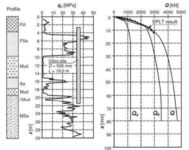
Figure 3. Example of Vibro pile calculation results obtained from load-transfer functions method (Gwizdala and Steczniewski 2007)
