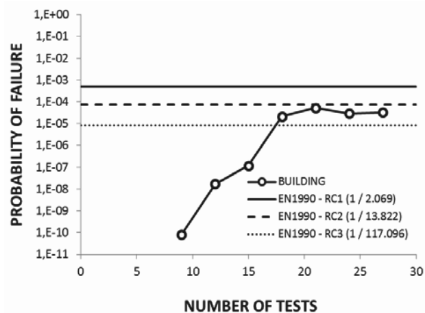
Figure 5. Variation of the probability of failure with an increase in the number of load tests.
