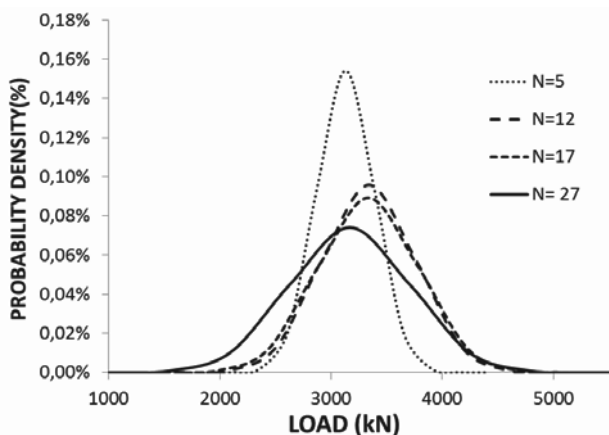
Figure 3. Standard curves varying according to the number of load tests analyzed.
