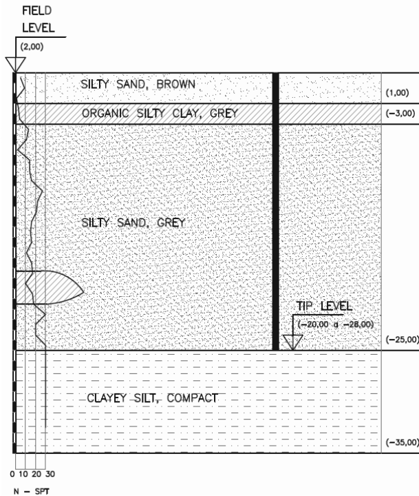
Figure 1. Subsoil profile
