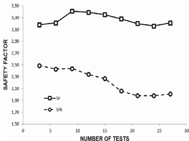
Figure 4. Variation of global and partial safety factors relative to the number of load tests.
