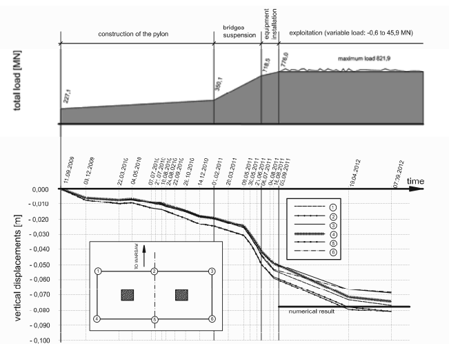
Figure 9: Settlements of foundation slab measured in 6 points in different phases of pylon loading.
