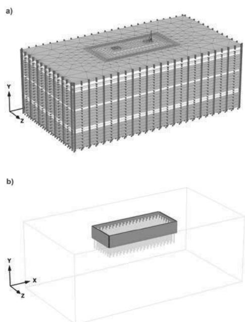
Figure 4: 3D FEM mesh of foundation model: a) general view with boundary conditions, b) detail of pile elements (so called embedded piles) and sheet pile wall elements (plate elements). Foundation body modelled by continuum elements.
