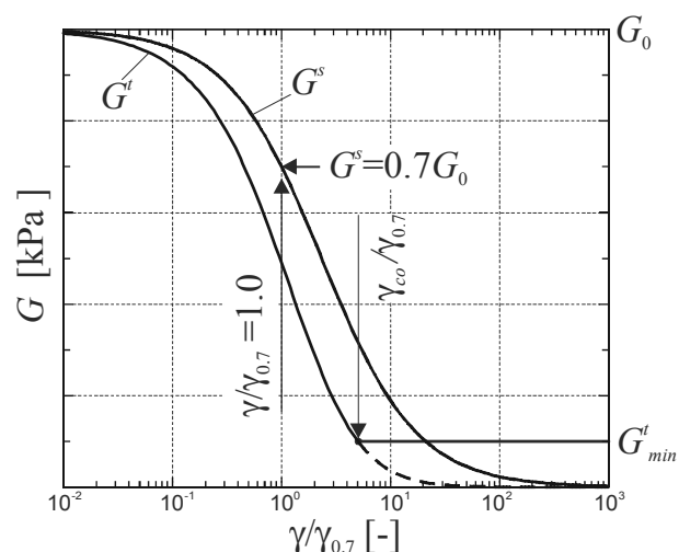
Figure 5: Dependence of shear modulus on shear strains. G_t = G_{ref} and G_s are tangent and secant shear moduli, respectively and G_{min} is a minimal shear modulus at the accumulation of shear strain \gamma_{co} .
