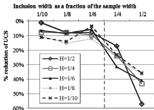
Figure 4. Influence of the dimensions of the soil inclusions on the UCS of soil mix material. Results of 2D numerical simulations performed with the help of the Universal Distinct Element Code UDEC of Itasca®. Details of the model are available in Van Lysebetten et al. (2013). H is the ratio between the height of the soil inclusion width and the sample diameter.
