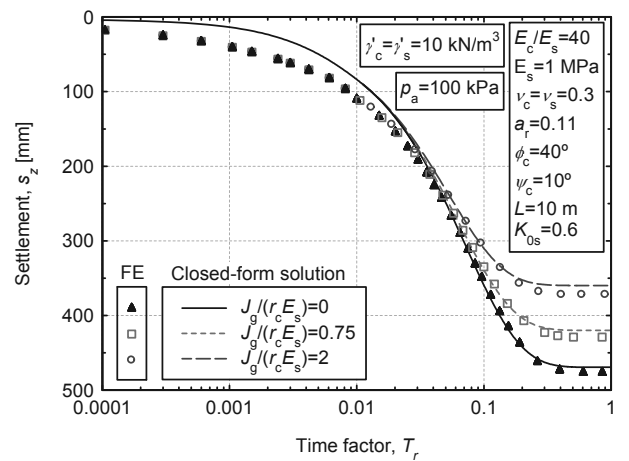
Figure 6. Time-settlement curve.
