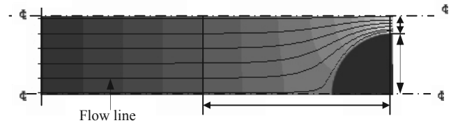
Figure 2. Calculating bulk wall permeability, k_p and flow-paths.
