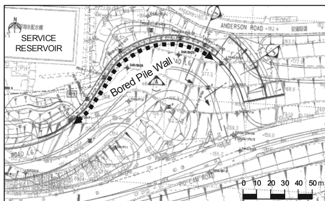
Figure 2. Layout of the bored pile wall with adjacent constraints
