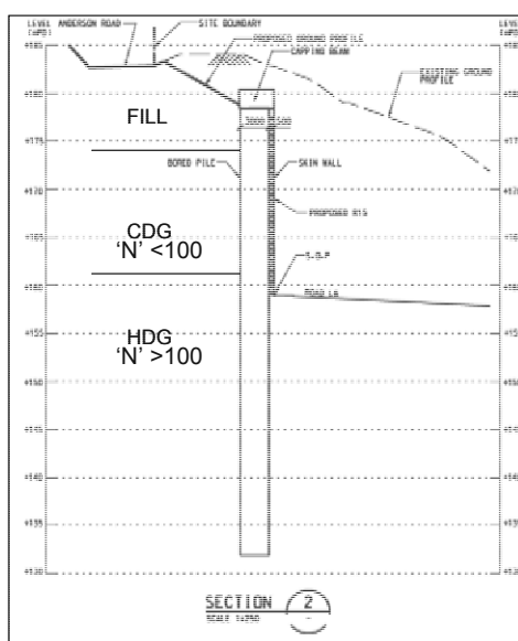
Figure 3. Geological section
