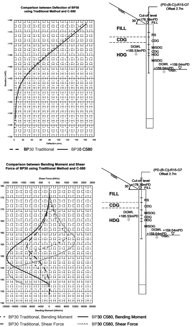
Figure 6. Calculated deflection, bending moment and shear force along cantilever bored pile wall (BP30)
