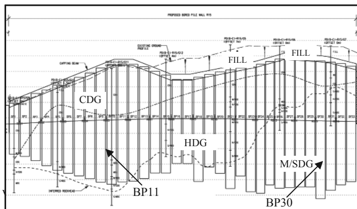
Figure 4. Geological long section
