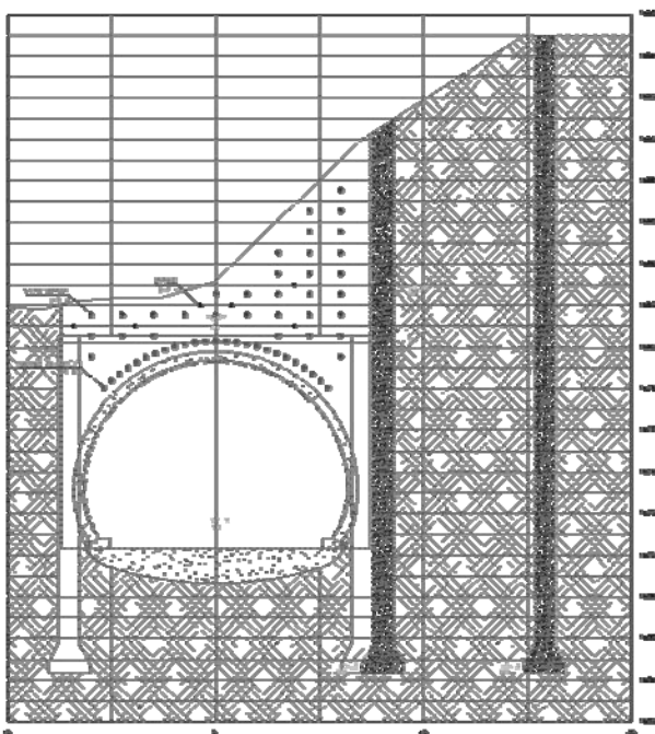
Figure 2. Section A-A, (see Figure 1)
