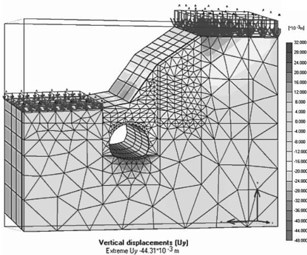
Figure 4. After construction settlements
