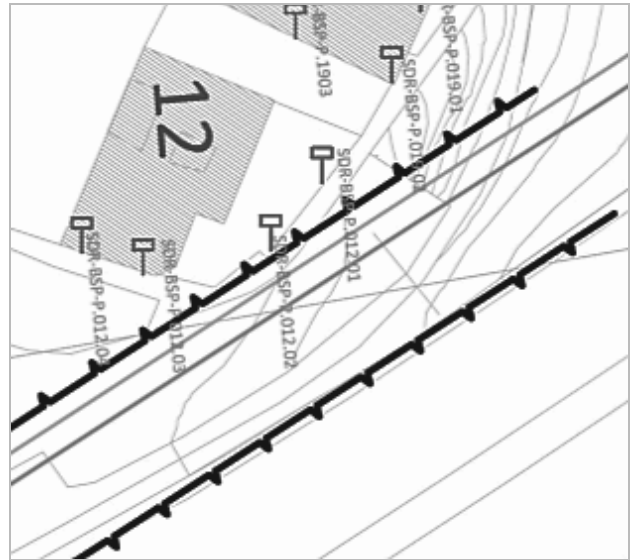
Figure 5. Settlements monitoring points
