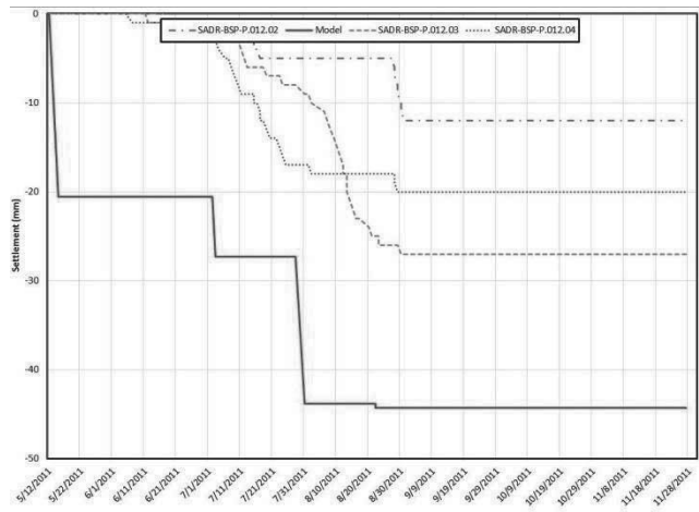
Figure 5. Settlements from monitoring and modeling
