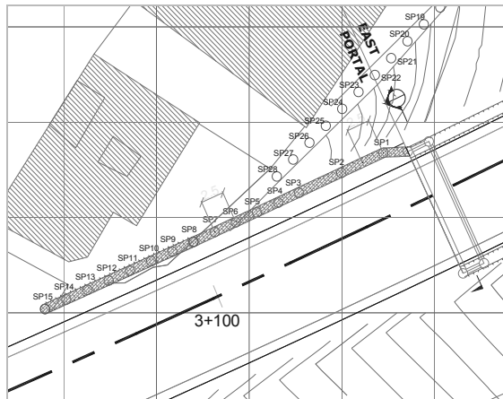
Figure 1. Plan of Niayesh east portal - north tunnel
