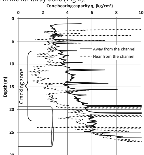
Figure 2. Soundings of piezocones carried out at the channel's zone of influence and away from it.
