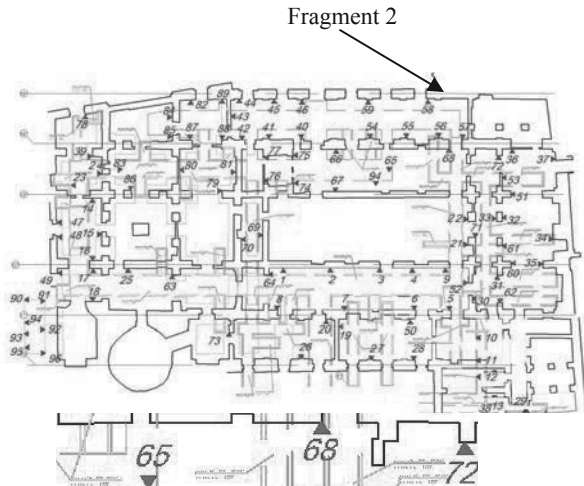
Figure 9 Geodetic markers layout and check markers 56, 57, 58 layout fragment
