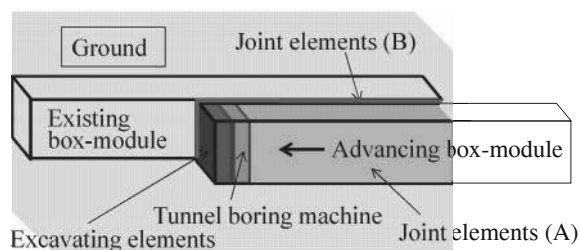
Figure 5. Arrangement of joint elements.
