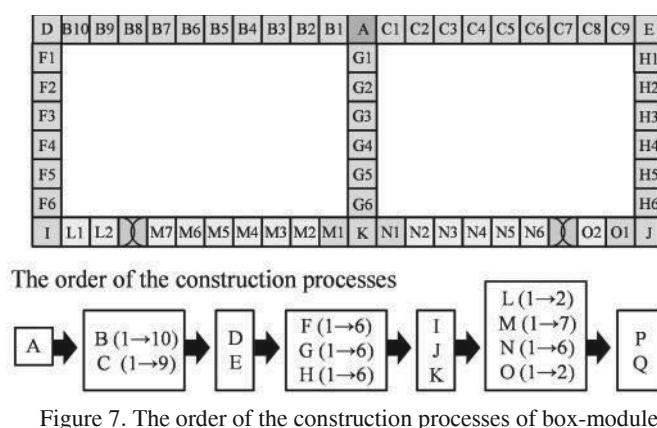
Figure 7. The order of the construction processes of box-module.
