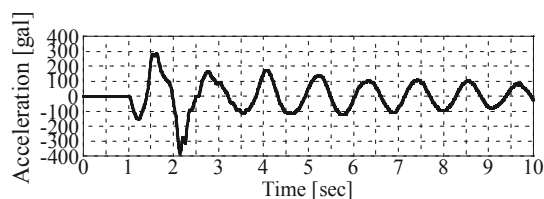
Figure 4. Input wave
