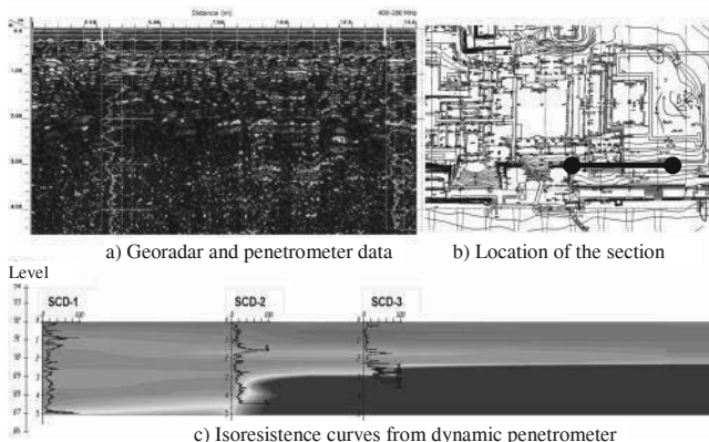
Figure 3 Typical results of the exploration with Georadar and Dynamic Penetrometer.
