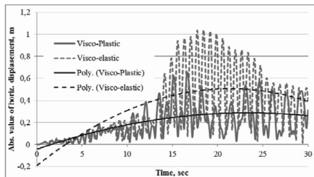
Figure 7. The diagram of absolute value of displacements for upper foundation slab (visco-elastoplastic model) and grillage slab (visco-elastic model)
