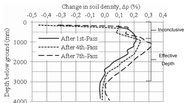
Figure 5. FEM predicted change in soil density versus depth after single and multiple passes.
