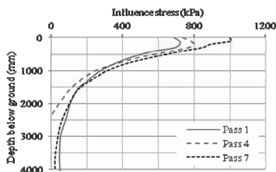
Figure 6. Influence stress versus depth for single and multiple passes.
