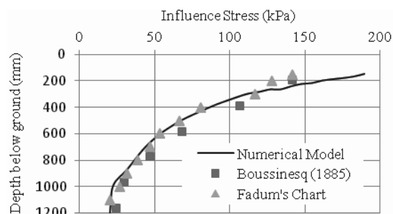
Figure 3. Validation of FEM model – static case.
