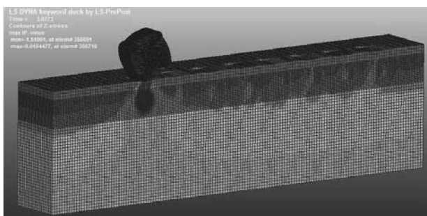
Figure 2. FEM model.
