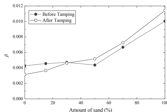
Figure 18. Relationships of \beta and % sand
