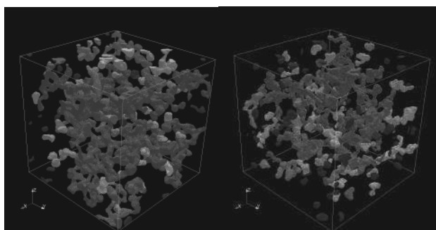
(a) Pore with LNAPL in Case 1 (b) Pore with LNAPL in Case 2 Figure 11. 3D MXCT images of isolated pore structures
